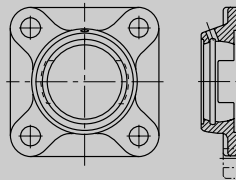
F Housing
